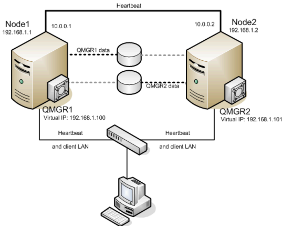
Figure 9 Active/Active Configuration with Shared Storage
