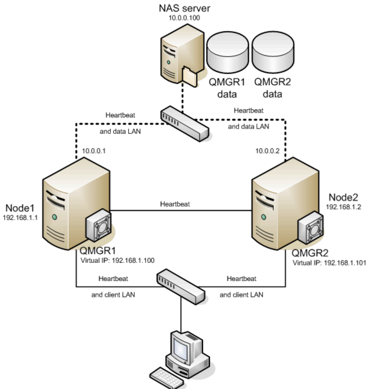
Figure 10 Active/Active Configuration with NFS Storage
