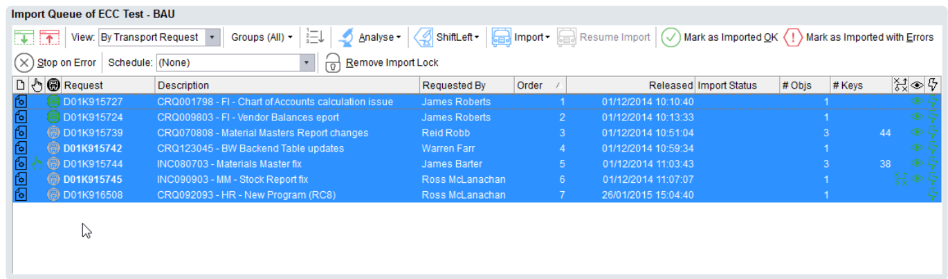
Figure: Copying data from ActiveControl Windows GUI using CTRL+A, CTRL+C
